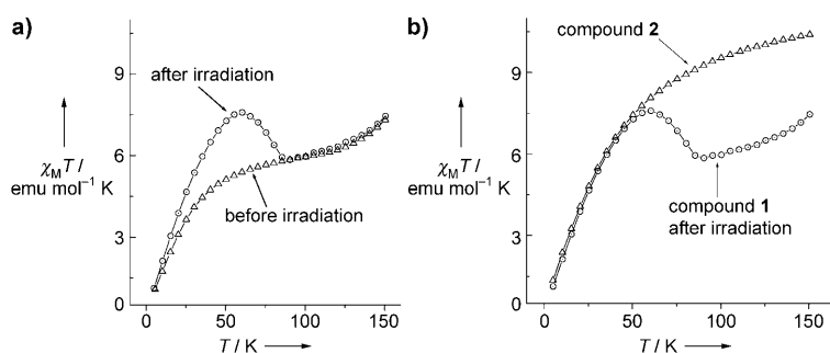
Figure 3. a) The photomagnetism of 1 (BF 4 ) 4 ; \Delta : \chi_M T per cluster before irradiation; \circ : \chi_M T upon warming after irradiation at \lambda = 785 \text{ nm} at 5 K for 30 min. b) Comparison of \chi_M T versus T for 2 (PF 6 ) 4 and 1 (BF 4 ) 4 after irradiation.
